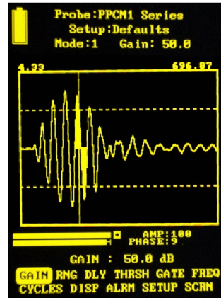
RF mode
