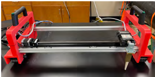
Motorized Axis Portable Scanner (MAPS) with AMWI System
